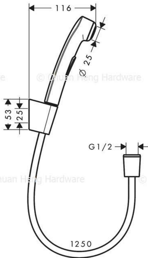
Bidette hand shower 1jet with shower holder and pressure shower hose 125 cm
